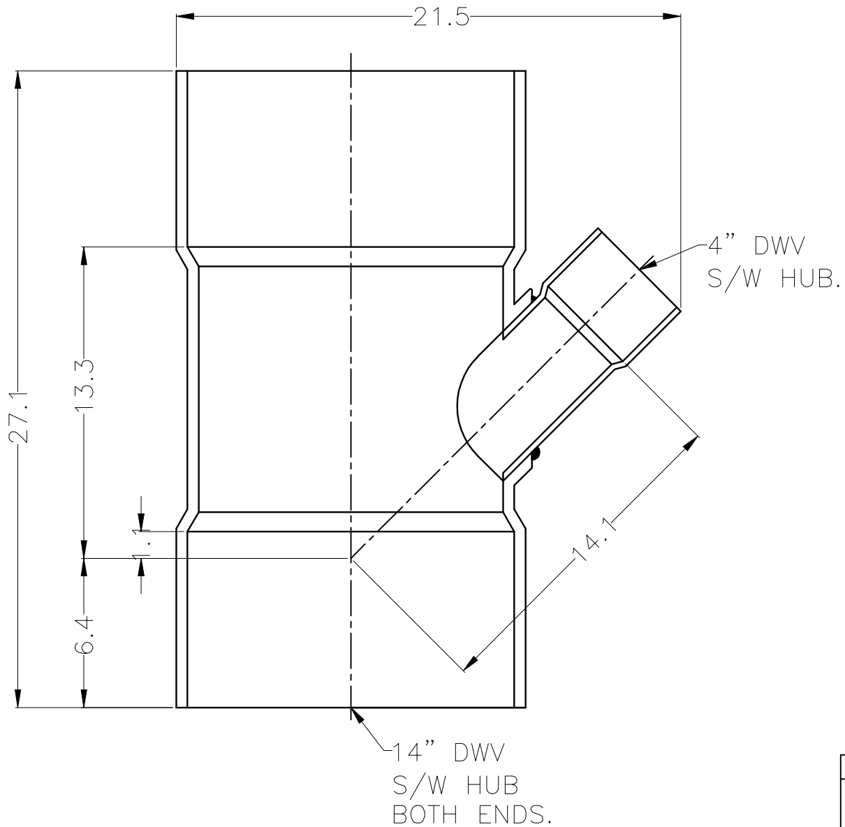
DWV 45 WYE 14X14X4
