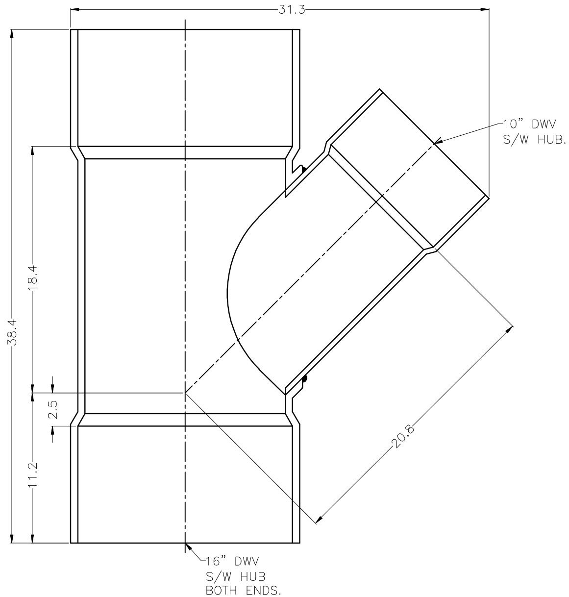
DWV 45 WYE 16X16X10
