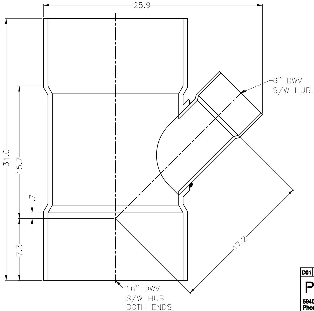
DWV 45 WYE 16X16X6
