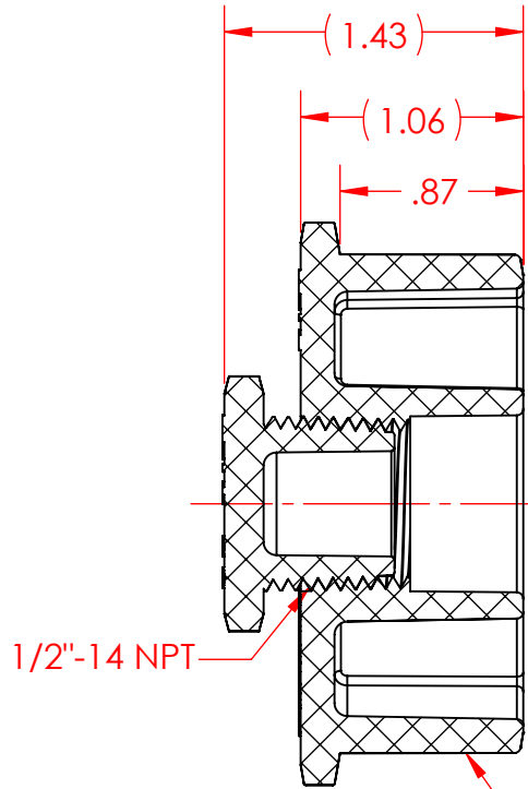
SECTION A-A 1/2"-14 NPT 2" TRADE SIZE SW DWV SPIGOT
