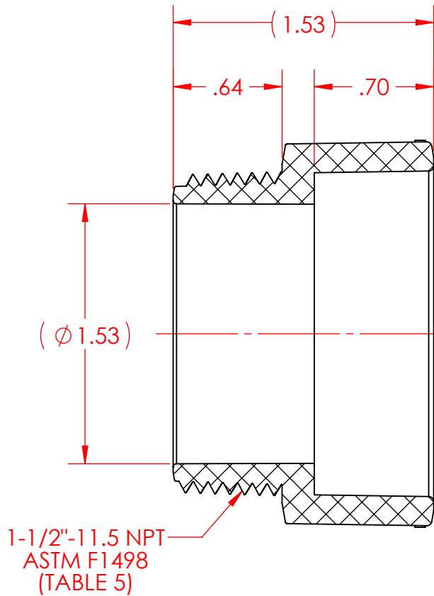
SECTION B-B
