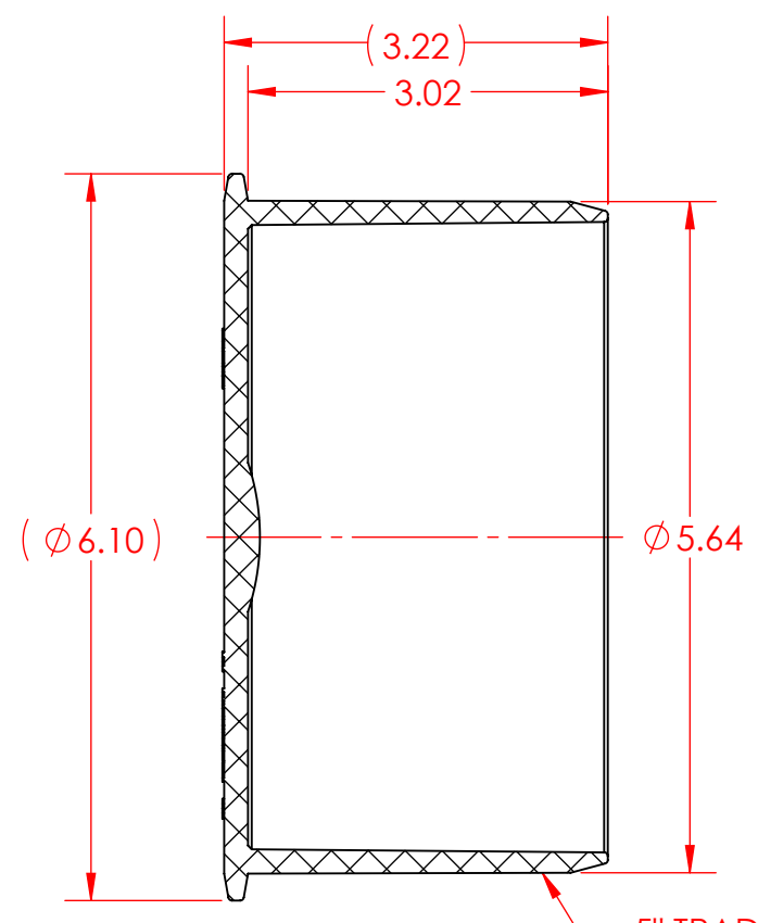
SECTION A-A 5" TRADE SIZE SDR35 SEWER SPIGOT
