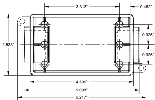
RFS10, RFS15 1/2", 3/4"
