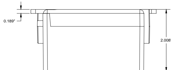
RFSC10, RFSC15 1/2", 3/4"
