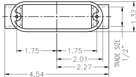
TOP VIEW W/O COVER
