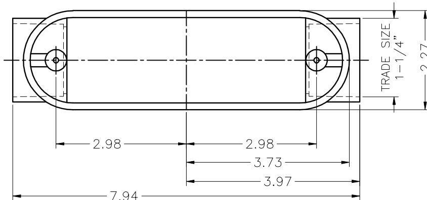
TOP VIEW W/O COVER
