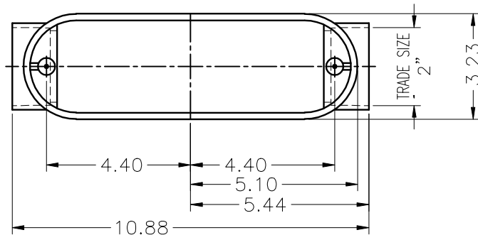
TOP VIEW W/O COVER
