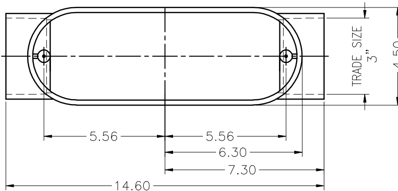
TOP VIEW W/O COVER
