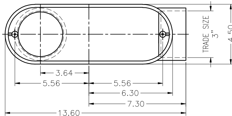
TOP VIEW W/O COVER
