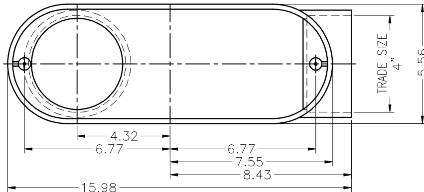
TOP VIEW W/O COVER
