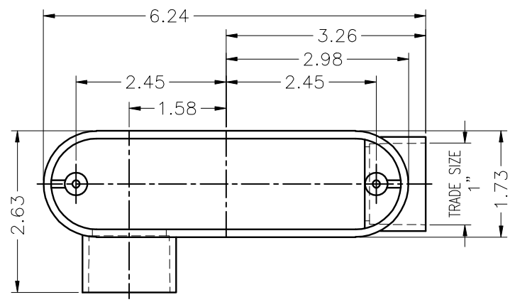
TOP VIEW W/O COVER
