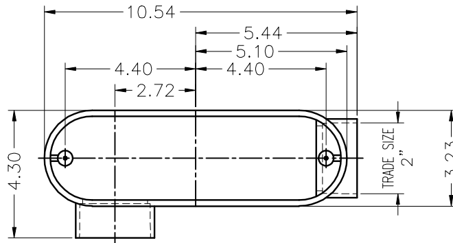
TOP VIEW W/O COVER
