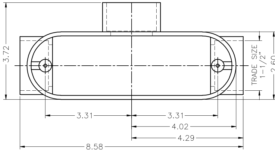
TOP VIEW W/O COVER
