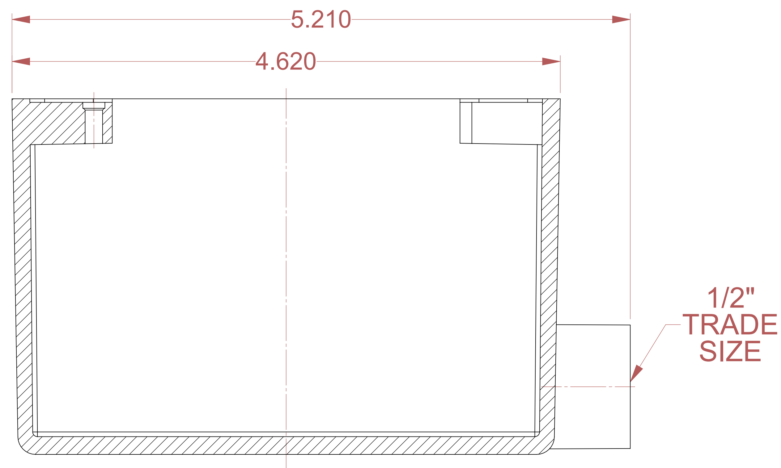
SECTION B-B
