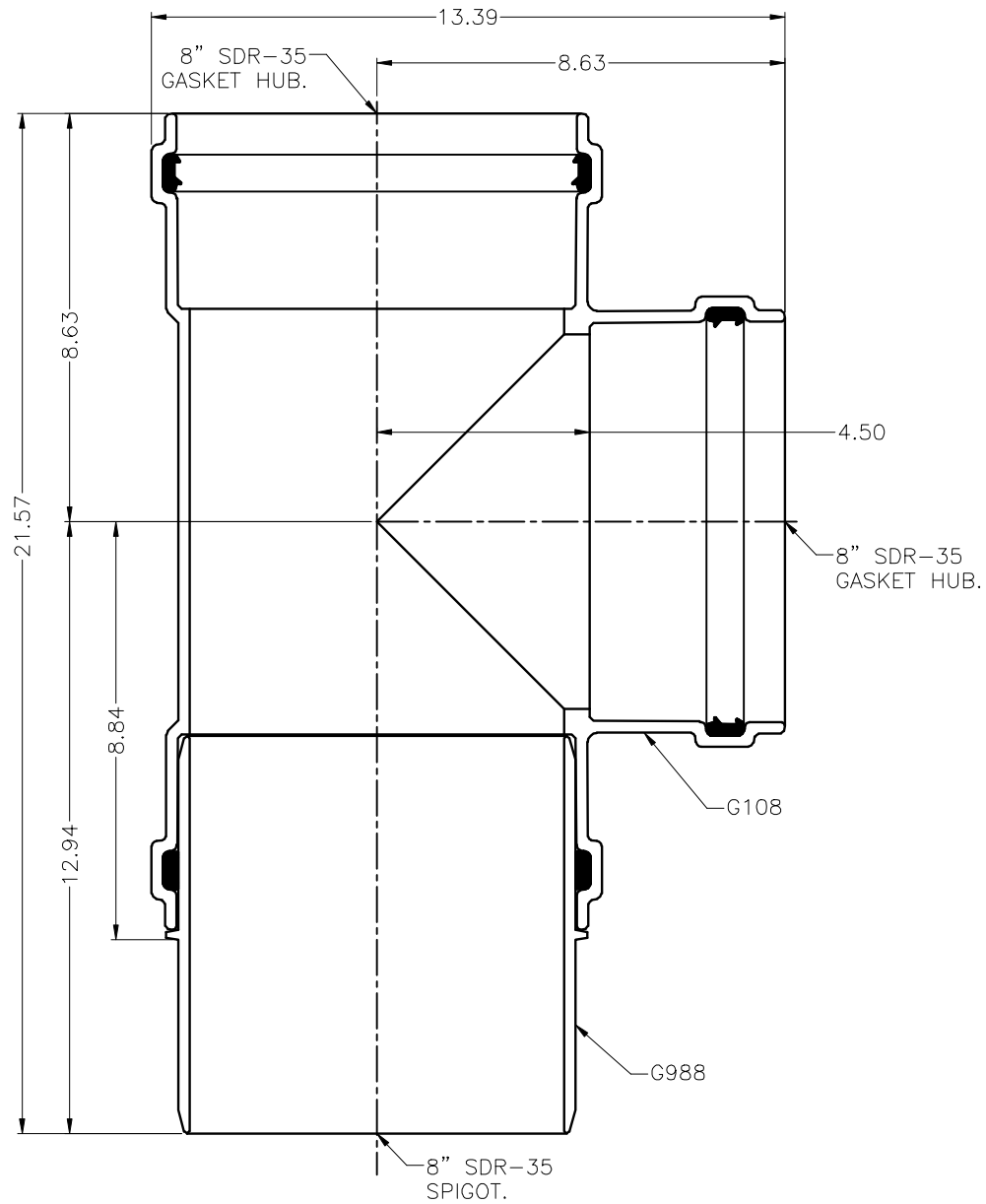
SDR 35 GASKET TEE SPIGOT 8X8X8
